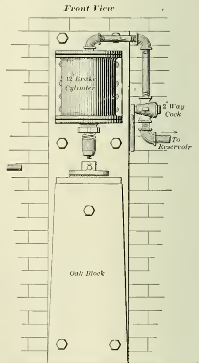
DEVICE FOR CUTTING GASKETS FROM OLD HOSE.
